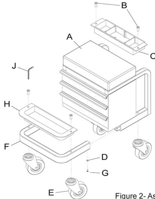
Figure 2- Assembly
